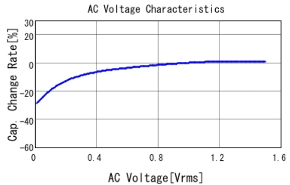
GCM188D70G106ME36 C-AC Voltage capchange, DCOV, 25.0d
