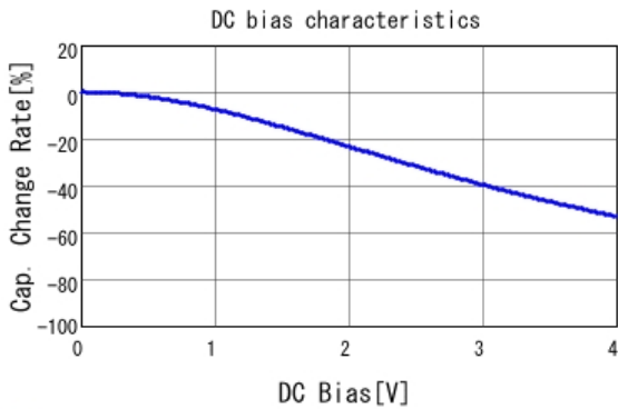
GCM188D70G106ME36 C-DC bias capchange, 25.0degC, AC1V
