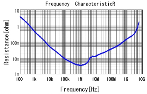
GCM188D70G106ME36 R DCOV, 25degC
