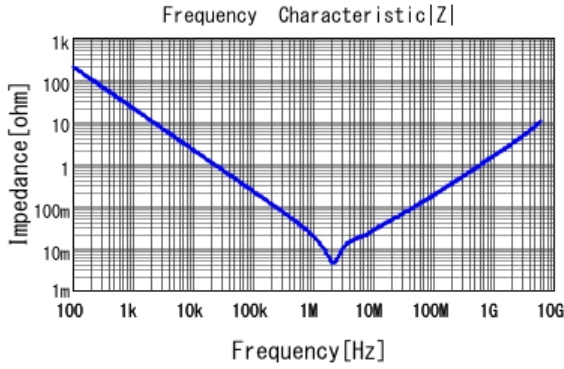
GCM188D70G106ME36 |Z| DCOV, 25degC
