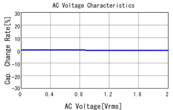
■ GCM1887U2A222JA16 C-AC Voltage capchange, DCOV, 25.0d
