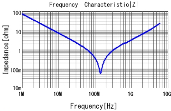
■ GCM1887U2A222JA16 |Z| DCOV, 25degC
