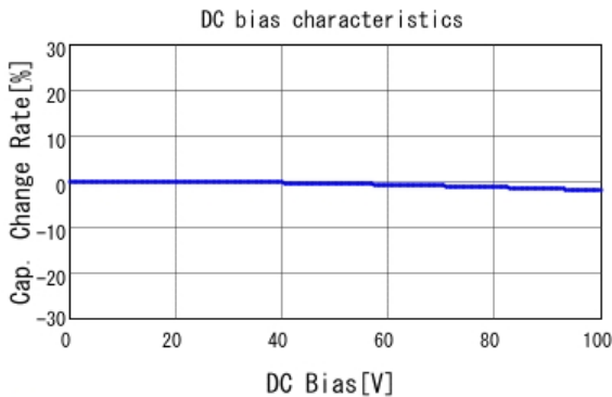
■ GCM1887U2A222JA16 C-DC bias capchange, 25.0degC, AC1V
