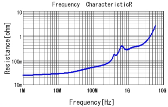
■ GCM1887U2A222JA16 R DCOV, 25degC
