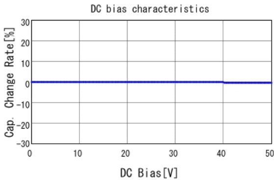
■ GCM1887U1H103JA16 C-DC bias capchange, 25.0degC, AC1V
