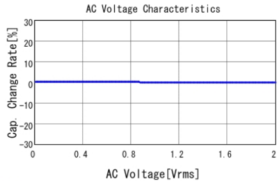
■ GCM1887U1H103JA16 C-AC Voltage capchange, DCOV, 25.0d
