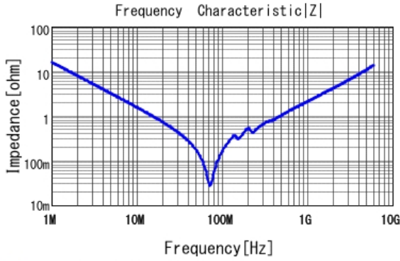
■ GCM1887U1H103JA16 |Z| DCOV, 25degC
