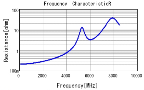
■ GCM1885C2A8R2DA16 R DCOV, 25degC
