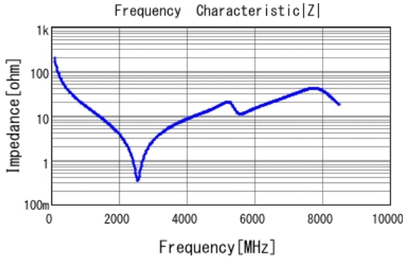
■ GCM1885C2A8R2DA16 |Z| DCOV, 25degC
