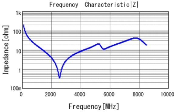
■ GCM1885C2A8R2BA16 |Z| DCOV, 25degC
