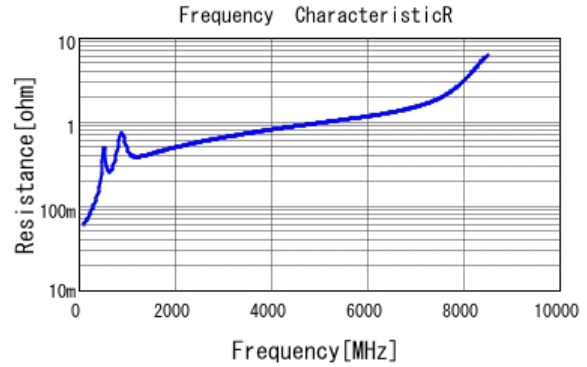
■ GCM1885C2A681JA16 R DCOV, 25degC
