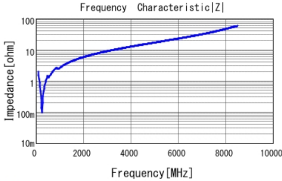
■ GCM1885C2A681JA16 |Z| DCOV, 25degC
