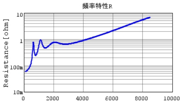
GCM1885C2A471JA16 R DCOV,25degC
