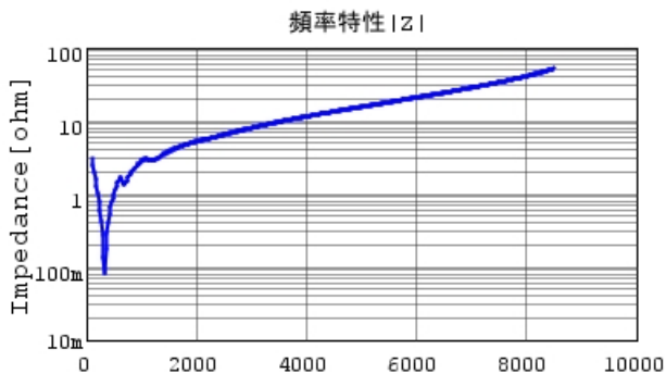
GCM1885C2A471JA16 |Z| DCOV,25degC
