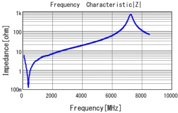
■ GCM1885C2A271JA16 |Z| DCOV, 25degC
