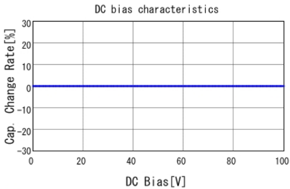
■ GCM1885C2A271JA16 C-DC bias capchange, 25.0degC, AC1V
