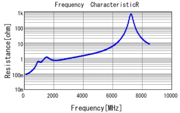
■ GCM1885C2A271JA16 R DCOV, 25degC
