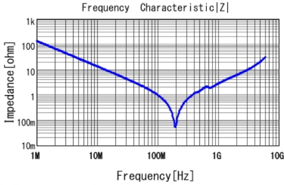
GCM1885C2A122JA16 |Z| DCOV, 25degC
