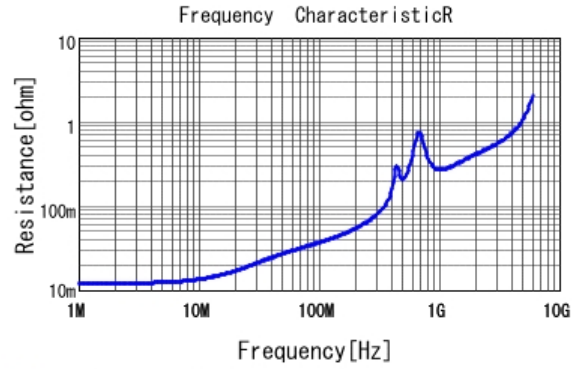
GCM1885C2A122JA16 R DCOV, 25degC
