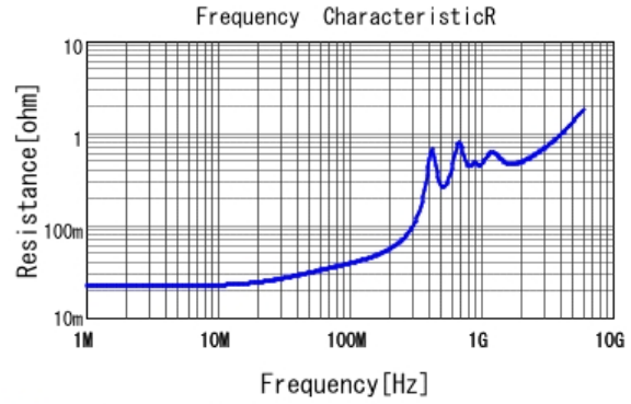
GCM1885C2A102JA16 R DCOV, 25degC
