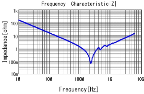
GCM1885C2A102JA16 |Z| DCOV, 25degC
