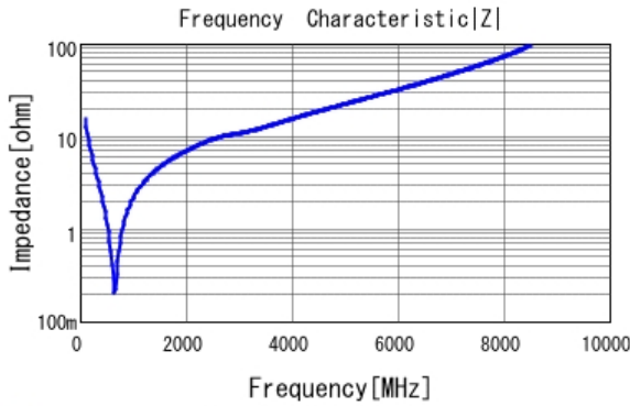
■ GCM1885C2A101JA16 |Z| DCOV, 25degC
