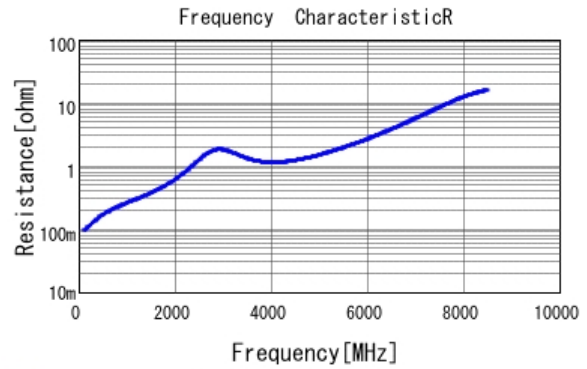
■ GCM1885C2A101JA16 R DCOV, 25degC
