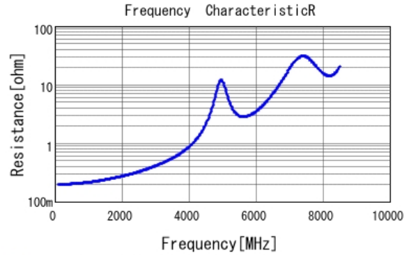
■ GCM1885C1H9R0DA16 R DCOV, 25degC
