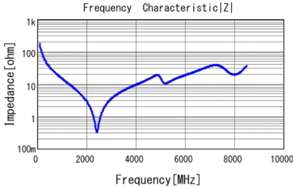
■ GCM1885C1H9R0DA16 |Z| DCOV, 25degC
