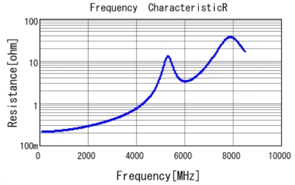
■ GCM1885C1H8R2DA16 R DCOV, 25degC
