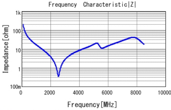
■ GCM1885C1H8R2DA16 |Z| DCOV, 25degC
