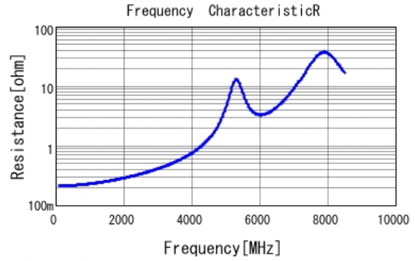
■ GCM1885C1H8R2BA16 R DCOV, 25degC
