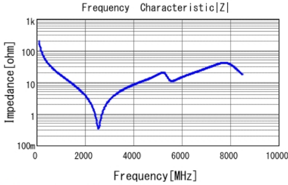
■ GCM1885C1H8R2BA16 |Z| DCOV, 25degC
