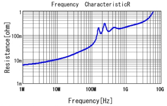
■ GCM1885C1H822JA16 R DCOV, 25degC
