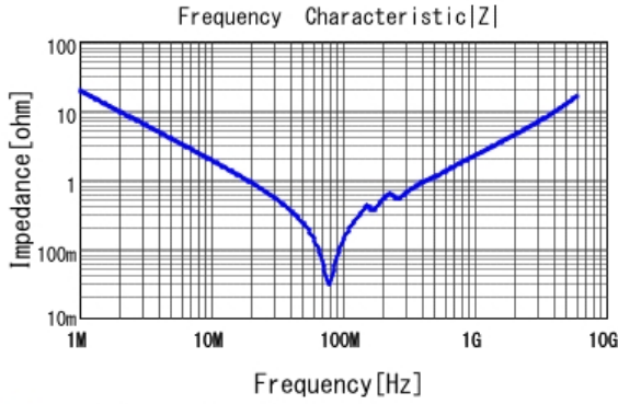
■ GCM1885C1H822JA16 |Z| DCOV, 25degC
