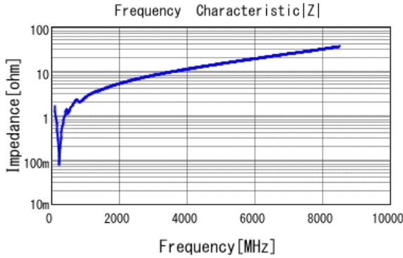
■ GCM1885C1H821JA16 |Z| DCOV, 25degC
