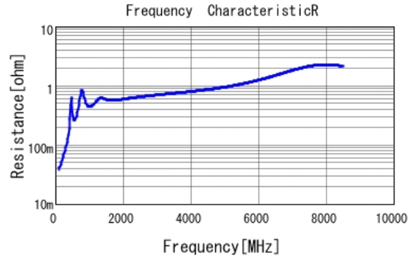
■ GCM1885C1H821JA16 R DCOV, 25degC
