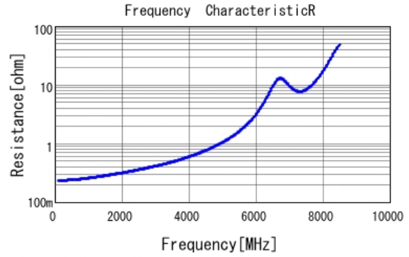
■ GCM1885C1H6R0BA16 R DCOV, 25degC
