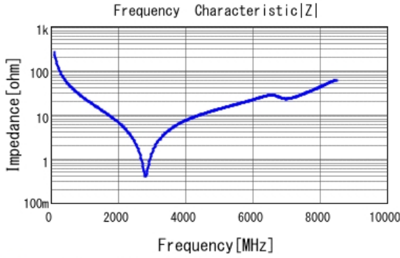
■ GCM1885C1H6R0BA16 |Z| DCOV, 25degC
