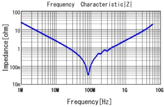
GCM1885C1H682JA16 |Z| DCOV, 25degC
