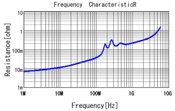
GCM1885C1H682JA16 R DCOV, 25degC
