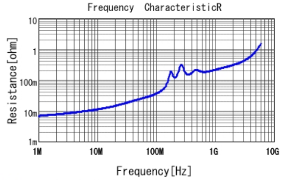
GCM1885C1H682GA16 R DCOV, 25degC
