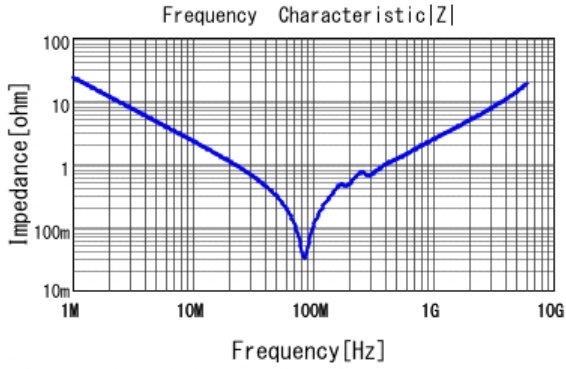
GCM1885C1H682GA16 |Z| DCOV, 25degC
