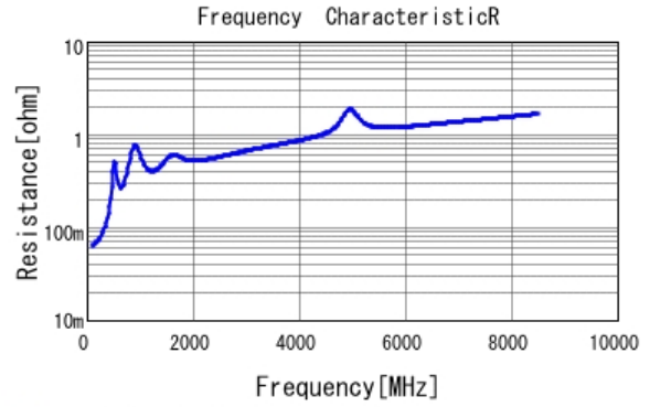
■ GCM1885C1H681JA16 R DCOV, 25degC
