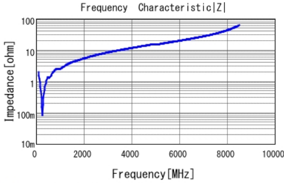
■ GCM1885C1H681JA16 |Z| DCOV, 25degC
