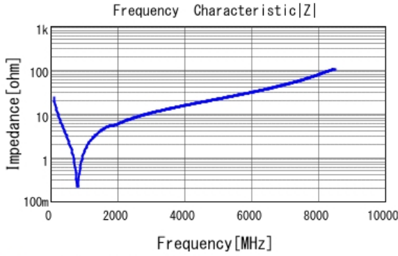
■ GCM1885C1H680JA16 |Z| DCOV, 25degC
