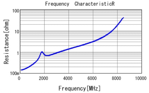
■ GCM1885C1H680JA16 R DCOV, 25degC
