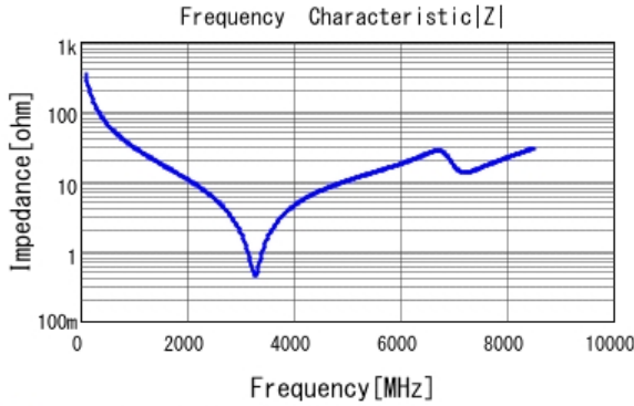
■ GCM1885C1H4R7CA16 |Z| DC0V, 25degC
