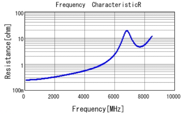
■ GCM1885C1H4R7CA16 R DC0V, 25degC
