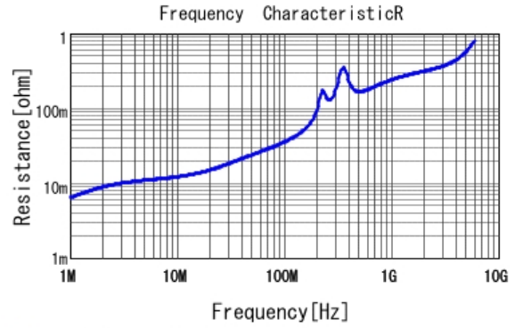
■ GCM1885C1H472JA16 R DCOV, 25degC
