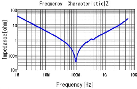
■ GCM1885C1H472JA16 |Z| DCOV, 25degC
