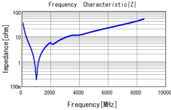
■ GCM1885C1H470JA16 |Z| DCOV, 25degC
