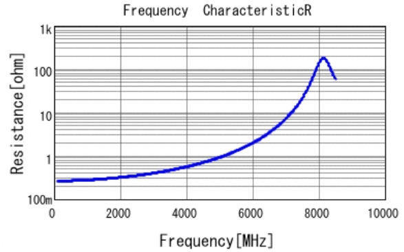
■ GCM1885C1H3R3CA16 R DCOV, 25degC
