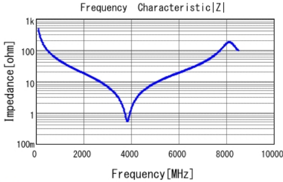
■ GCM1885C1H3R3CA16 |Z| DCOV, 25degC
