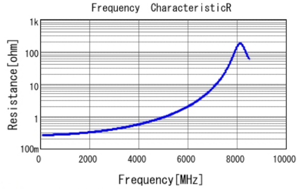
■ GCM1885C1H3R3BA16 R DCOV, 25degC
