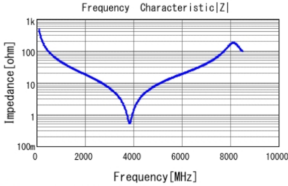
■ GCM1885C1H3R3BA16 |Z| DCOV, 25degC
