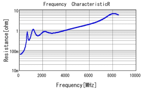
■ GCM1885C1H391JA16 R DCOV, 25degC
