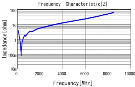
■ GCM1885C1H391JA16 |Z| DCOV, 25degC
