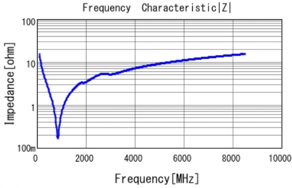
■ GCM1555G1H101JA16 |Z| DCOV, 25degC
