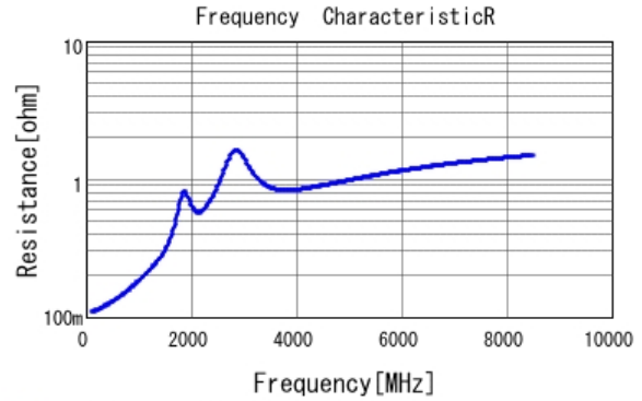
■ GCM1555G1H101FA16 R DCOV, 25degC
