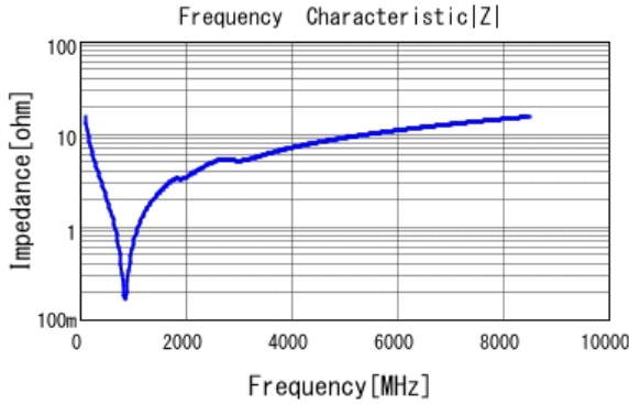
■ GCM1555G1H101FA16 |Z| DCOV, 25degC
