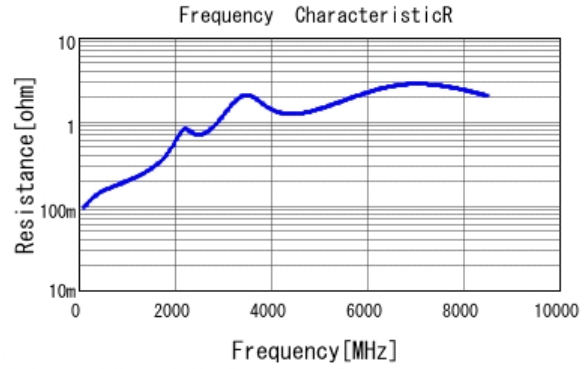
■ GCM1555C1H820JA16 R DCOV, 25degC
