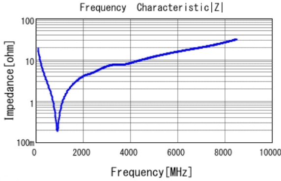
■ GCM1555C1H820JA16 |Z| DCOV, 25degC
