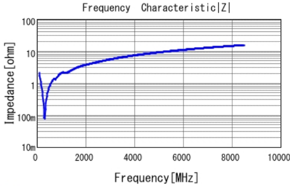
■ GCM1555C1H681FA16 |Z| DCOV, 25degC
