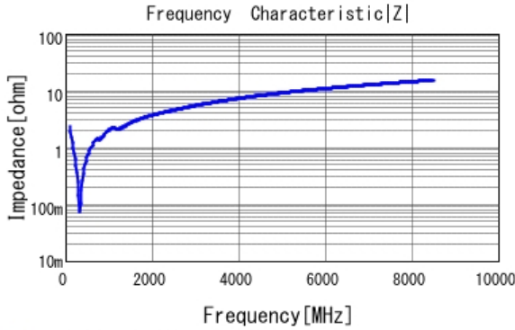
■ GCM1555C1H621FA16 |Z| DCOV, 25degC
