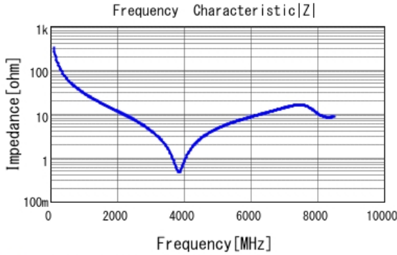
GCM1555C1H5R0FA16 |Z| DCOV, 25degC
