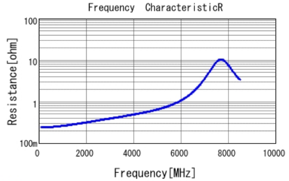
GCM1555C1H5R0FA16 R DCOV, 25degC
