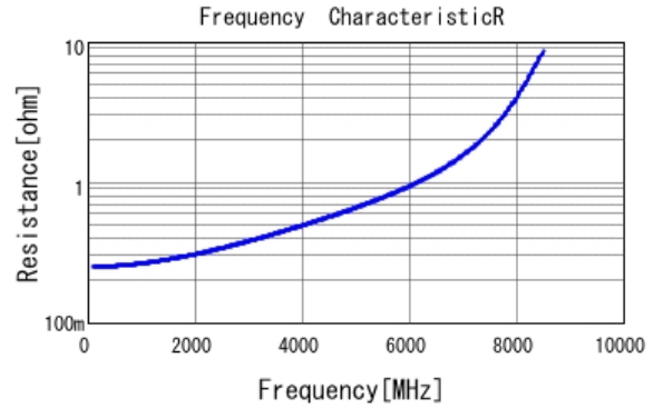
■ GCM1555C1H4R0BA16 R DCOV, 25degC
