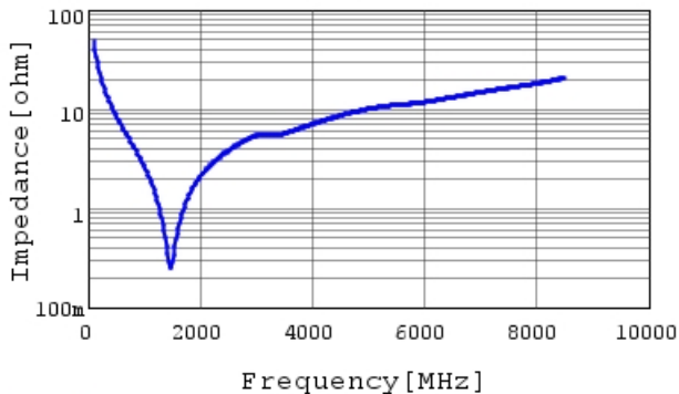
GCM1555C1H330JA16 |Z| DCOV,25degC
