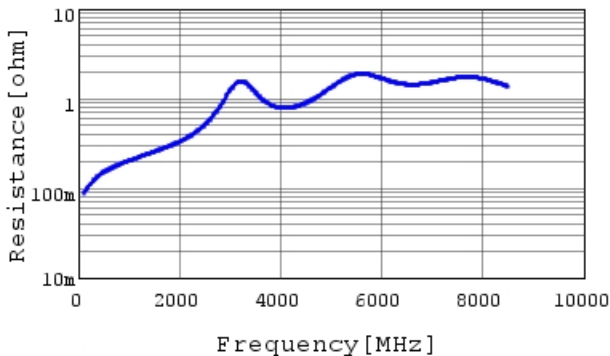
GCM1555C1H330JA16 R DCOV,25degC
