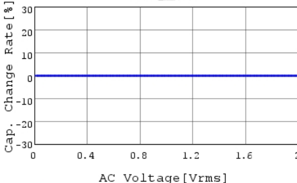
GCM1555C1H330JA16 C-AC Voltage capchange, DC
