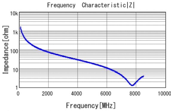
■ GCM1555C1H1R0JA16 |Z| DCOV, 25degC
