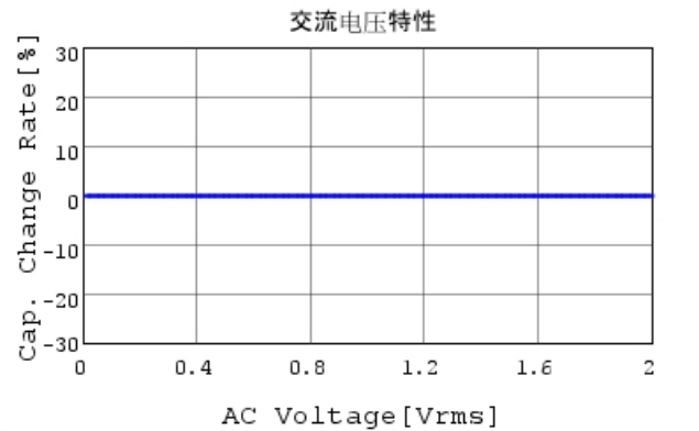
GCM1555C1H1R0CA16 C-AC Voltage capchange, DC
