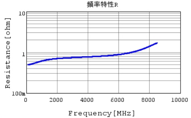
GCM1555C1H1R0CA16 R DCOV, 25degC
