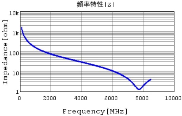
GCM1555C1H1R0CA16 |Z| DCOV, 25degC
