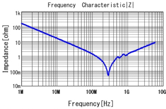
GCM1555C1H102JA16 |Z| DCOV, 25degC
