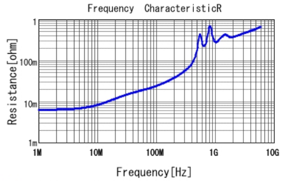
GCM1555C1H102JA16 R DCOV, 25degC
