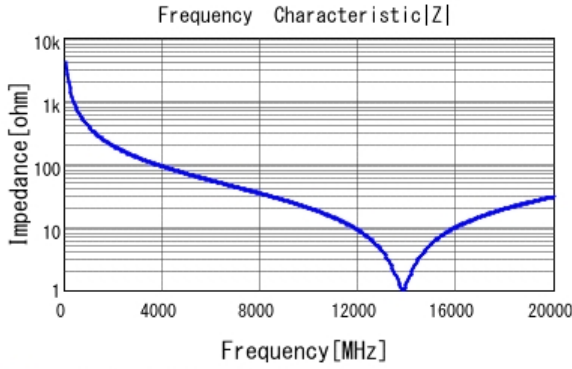
GCM0335C1HR40WA16 |Z| DCOV, 25degC
