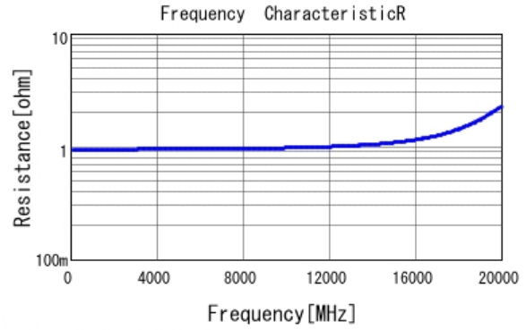
GCM0335C1HR40WA16 R DCOV, 25degC
