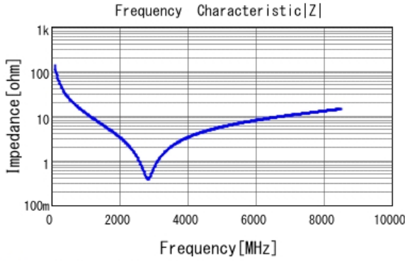
■ GCM0335C1H120JA16 |Z| DCOV, 25degC
