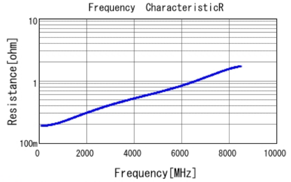
■ GCM0335C1H120JA16 R DCOV, 25degC
