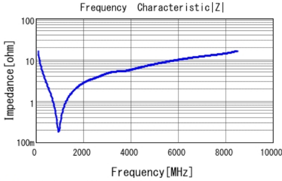
■ GCM0335C1H101FA16 |Z| DCOV, 25degC
