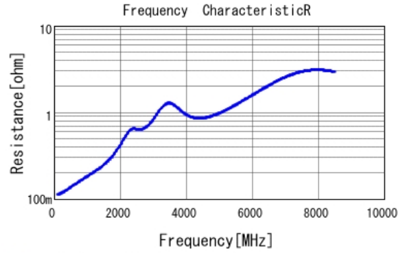
■ GCM0335C1H101FA16 R DCOV, 25degC
