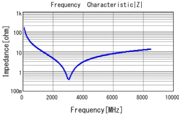
GCM0335C1H100GA16 |Z| DC0V, 25degC
