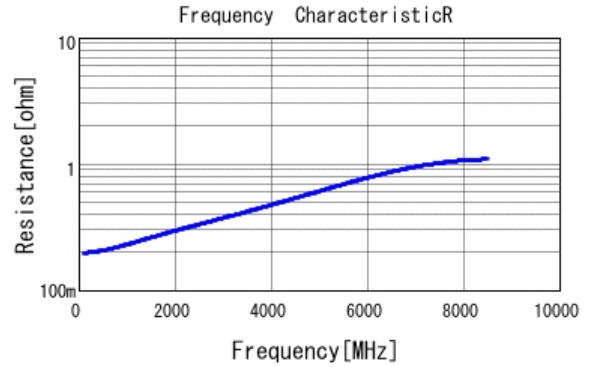
GCM0335C1H100GA16 R DC0V, 25degC
