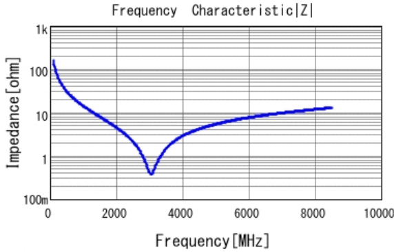
■ GCM0335C1H100FA16 |Z| DCOV, 25degC
