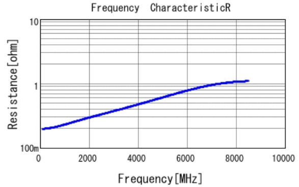
■ GCM0335C1H100FA16 R DCOV, 25degC
