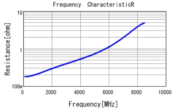
■ GCM0335C1E150FA16 R DCOV, 25degC
