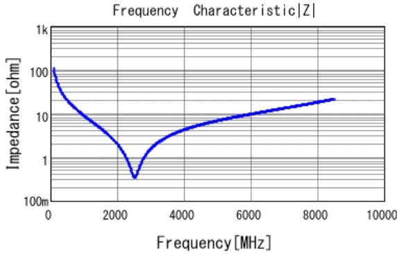
■ GCM0335C1E150FA16 |Z| DCOV, 25degC
