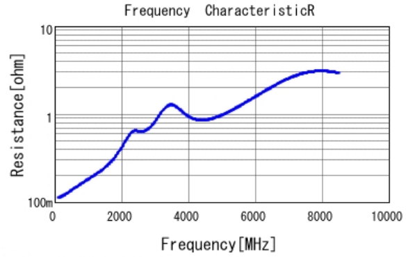
■ GCM0335C1E101GA16 R DCOV, 25degC
