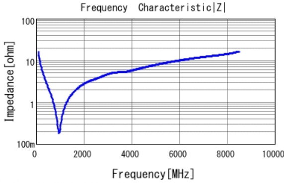
■ GCM0335C1E101GA16 |Z| DCOV, 25degC
