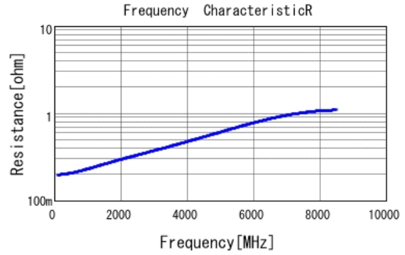
■ GCM0335C1E100JA16 R DCOV, 25degC
