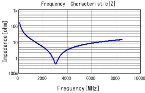
■ GCM0335C1E100JA16 |Z| DCOV, 25degC
