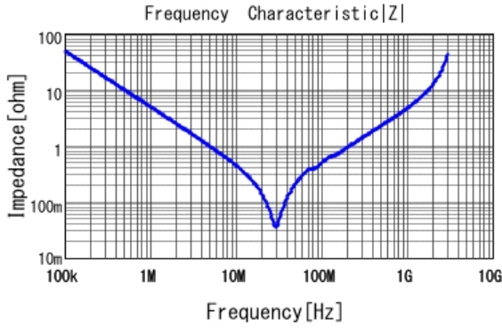
■ GCJ43DR72J333KXJ1 |Z| DC0V, 25degC
