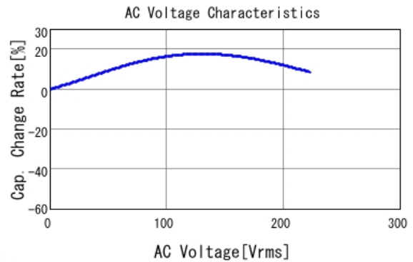
■ GCJ43DR72J333KXJ1 C-AC Voltage capchange, DC0V, 25.0d
