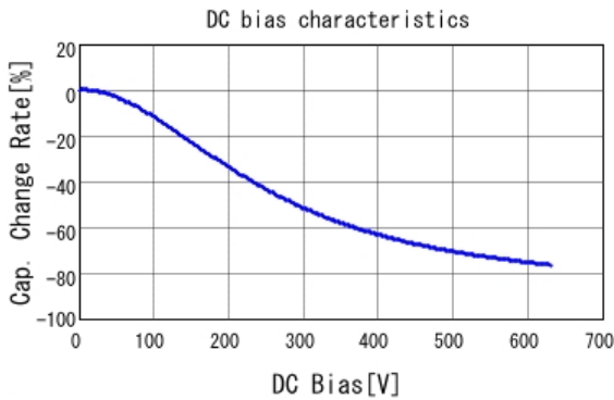
■ GCJ43DR72J333KXJ1 C-DC bias capchange, 25.0degC, AC1V
