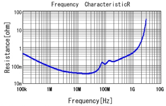
■ GCJ43DR72J333KXJ1 R DC0V, 25degC
