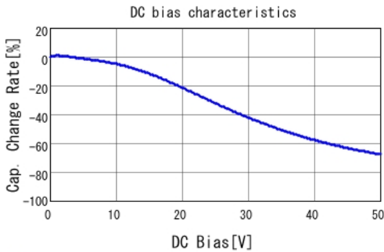
■ GCJ32ER71H475KA12 C-DC bias capchange, 25.0degC, AC1.
