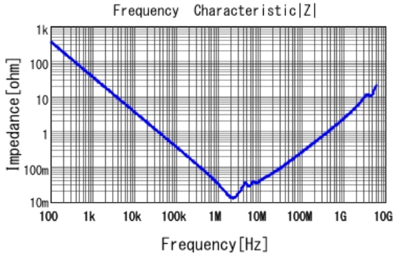
■ GCJ32ER71H475KA12 |Z| DC0V, 25degC
