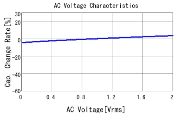
■ GCJ32ER71H475KA12 C-AC Voltage capchange, DC0V, 25.0d
