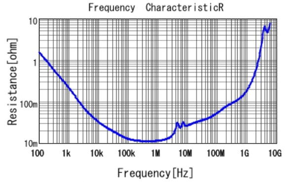
■ GCJ32ER71H475KA12 R DC0V, 25degC
