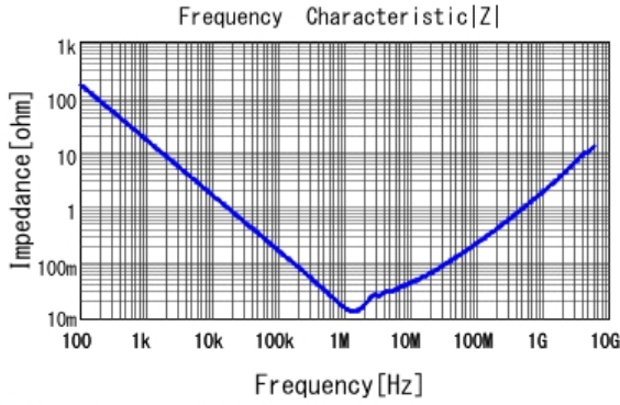
■ GCJ32EC71H106MA01 |Z| DC0V, 25degC
