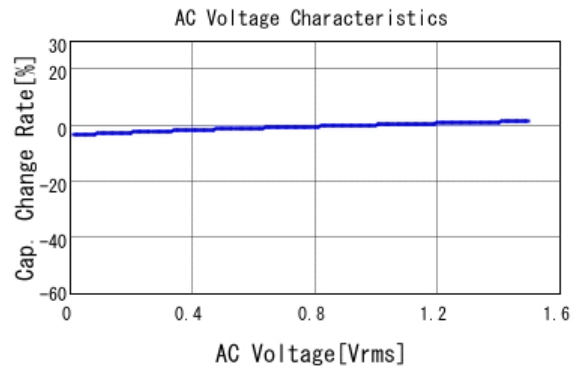
■ GCJ32EC71H106MA01 C-AC Voltage capchange, DC0V, 25.0d
