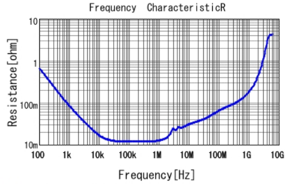
■ GCJ32EC71H106MA01 R DC0V, 25degC
