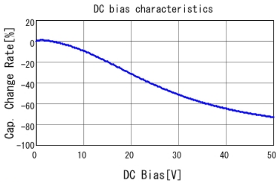
■ GCJ32EC71H106MA01 C-DC bias capchange, 25.0degC, AC1.
