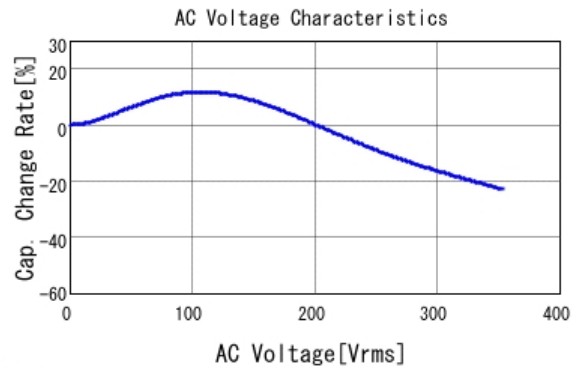
■ GCJ32DR73A223KXJ1 C-AC Voltage capchange, DC0V, 25.0d
